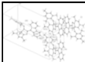
Fig. 2. The molecular packing of the title compound. Dashed lines indicate the C—H... \pi intramolecular contacts [Symmetry codes: (i) -x, -y, -z ; (ii) 1 + x, +y, +z ; (iii) 1/2 + x, 1/2 - y, 1/2 + z ].
