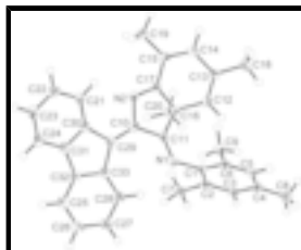
Fig. 1. The molecular structure of the title compound, showing the atom-labeling scheme. Displacement ellipsoids are drawn at the 50% probability level.
